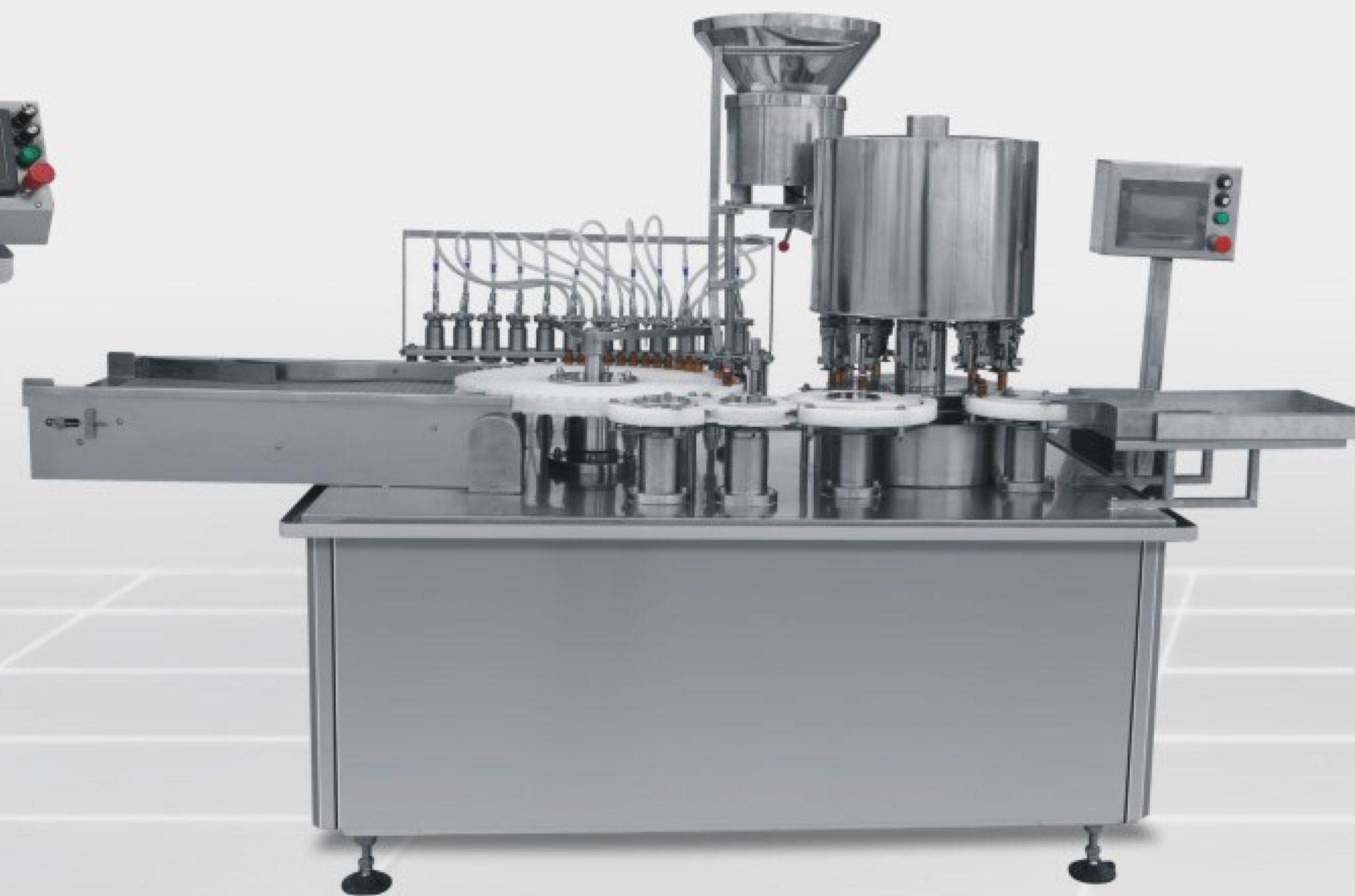
SGKGZ-12口服液灌装轧盖机 4 heads oral liquid filling capping machine
