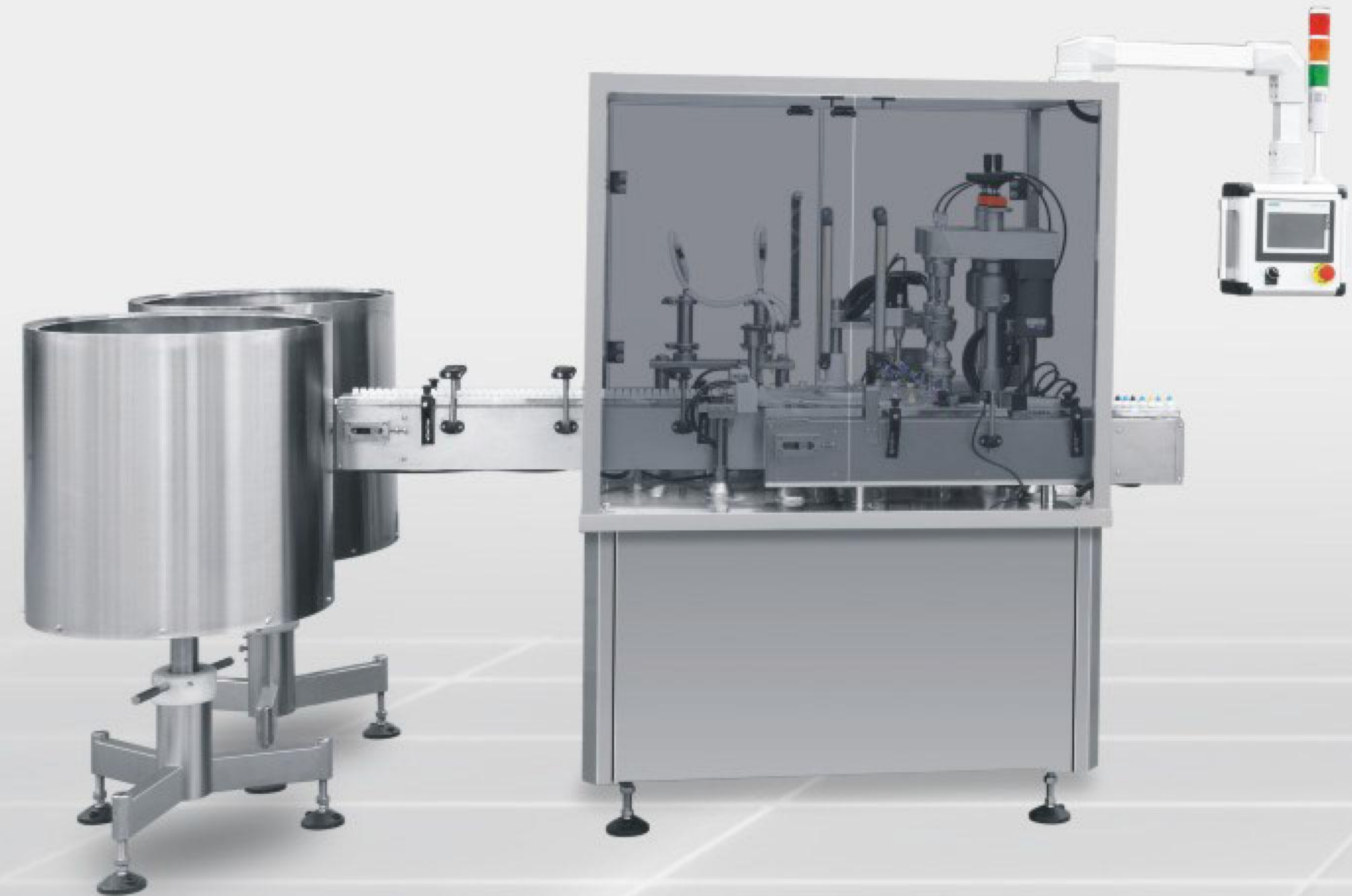
SGSJ型微量试剂灌装机 SGSJ-Micro reagent filling machine
